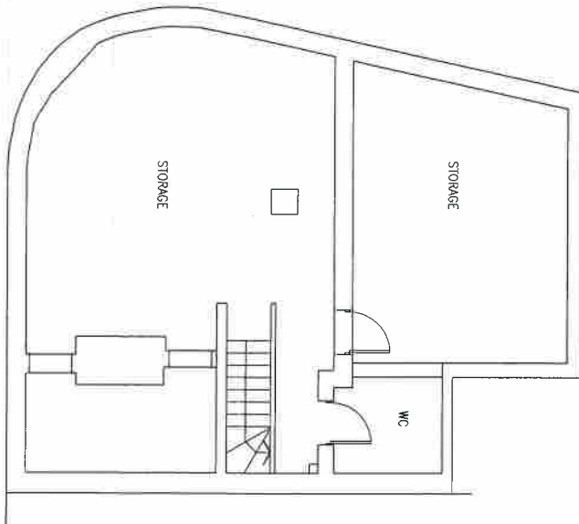
BASEMENT FLOOR PLAN SCALE 1:100 @A3
